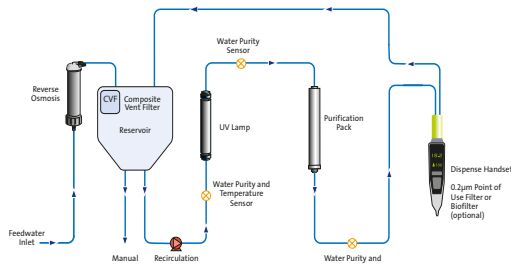
Process Flow PURELAB flex 3 Process Flow PURELAB flex 3
