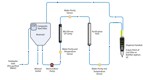
Process Flow PURELAB flex 4 Process Flow PURELAB flex 4
