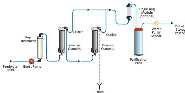
Process Flow PURELAB Chorus 2 (RO/DI)
